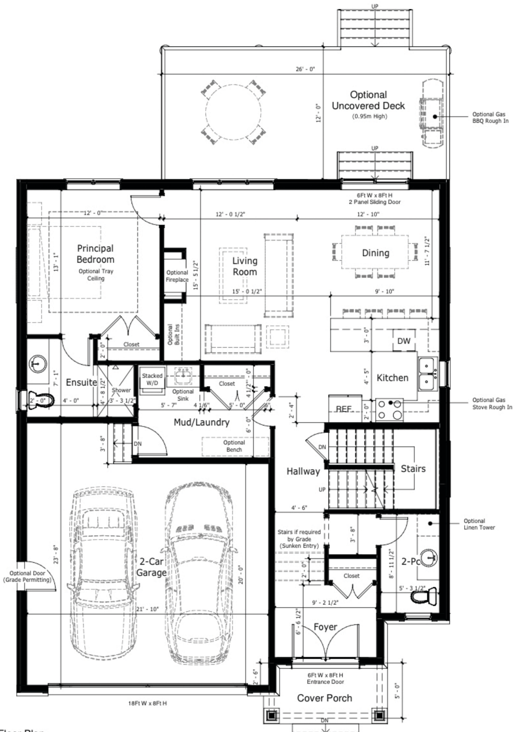
First Floor Plan 3/16" = 1'-0"
