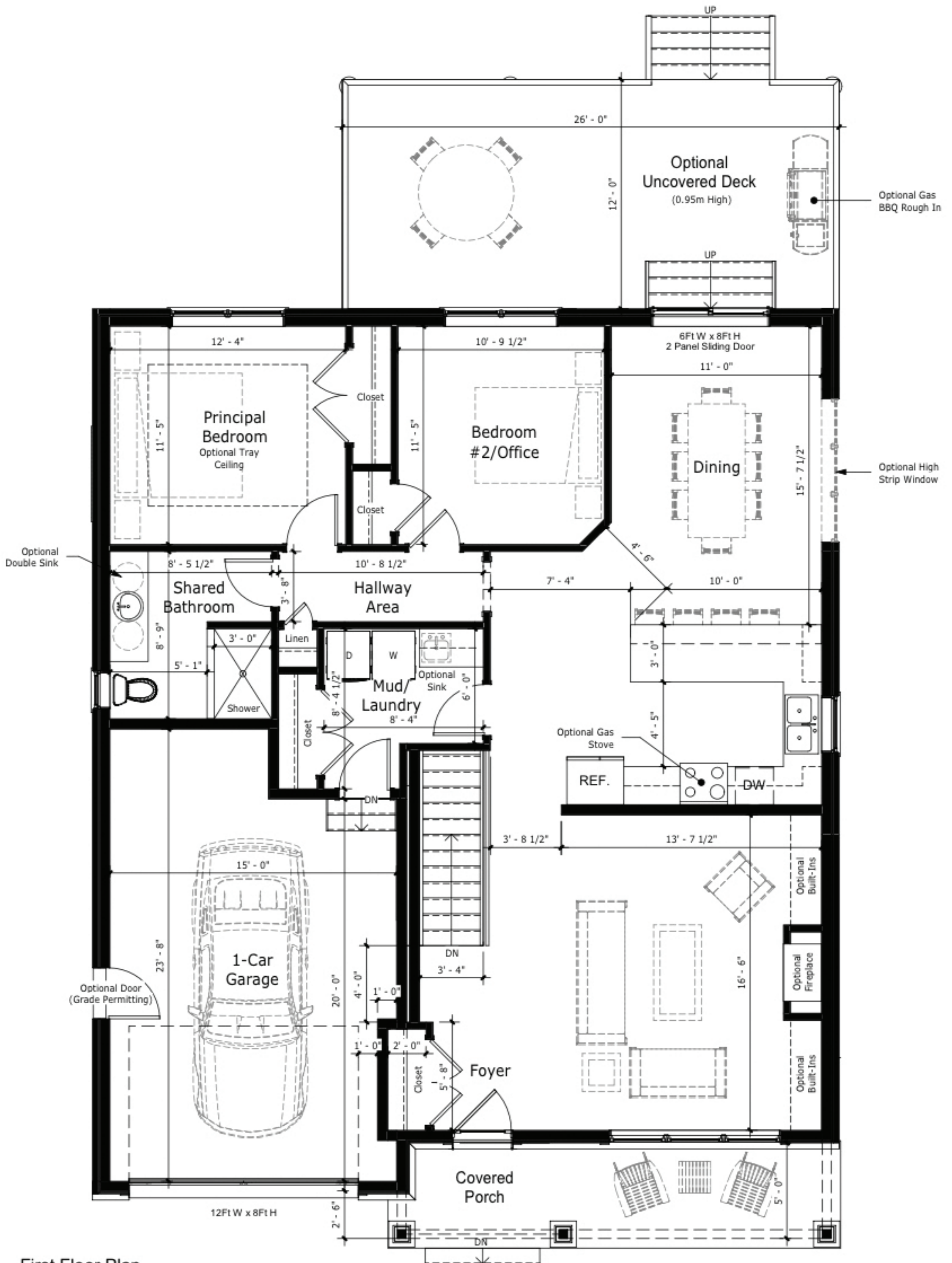
First Floor Plan 3/16" = 1'-0"
